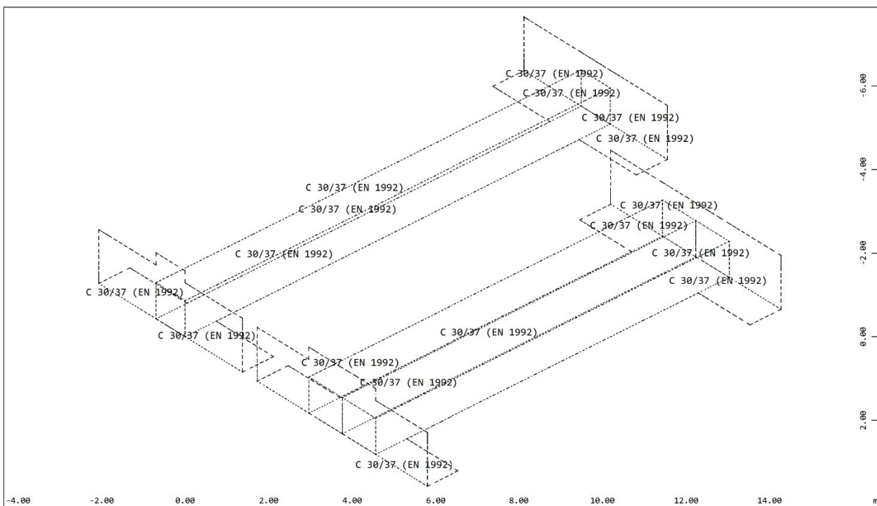
Quadrilateral Elements , Material designations
