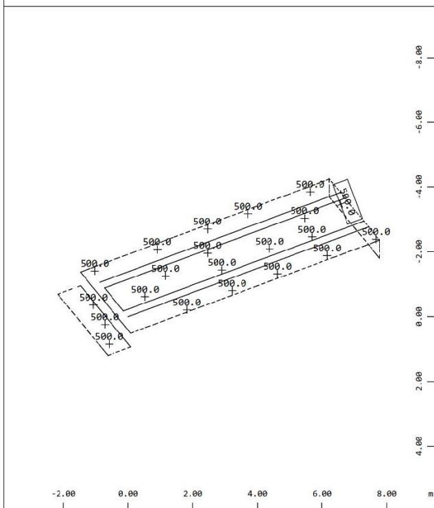
Sector of system Group 70 Quadrilateral Elements , Average plate thickness in mm (Max=500.0)
