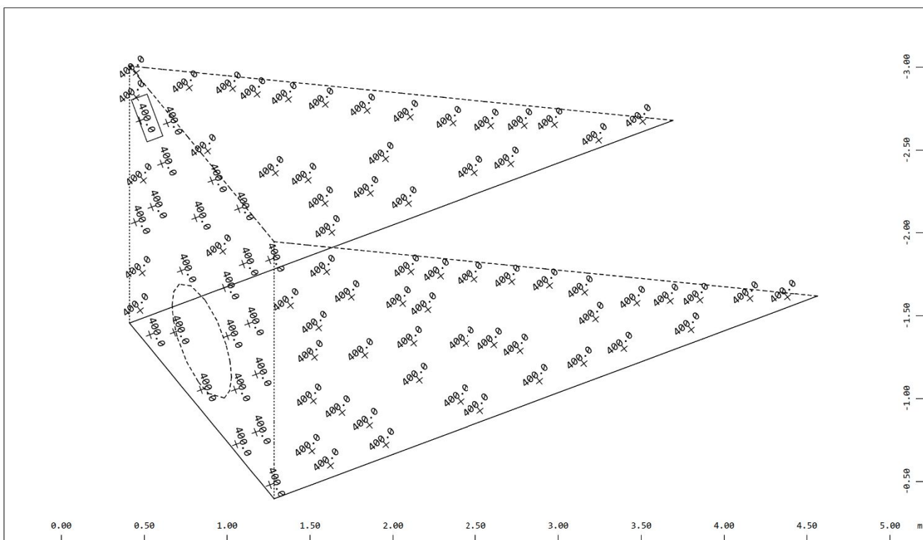
Sector of system Quadrilateral Elements Group 51...53 Quadrilateral Elements , Average plate thickness in mm (Max=400.0) Contour
