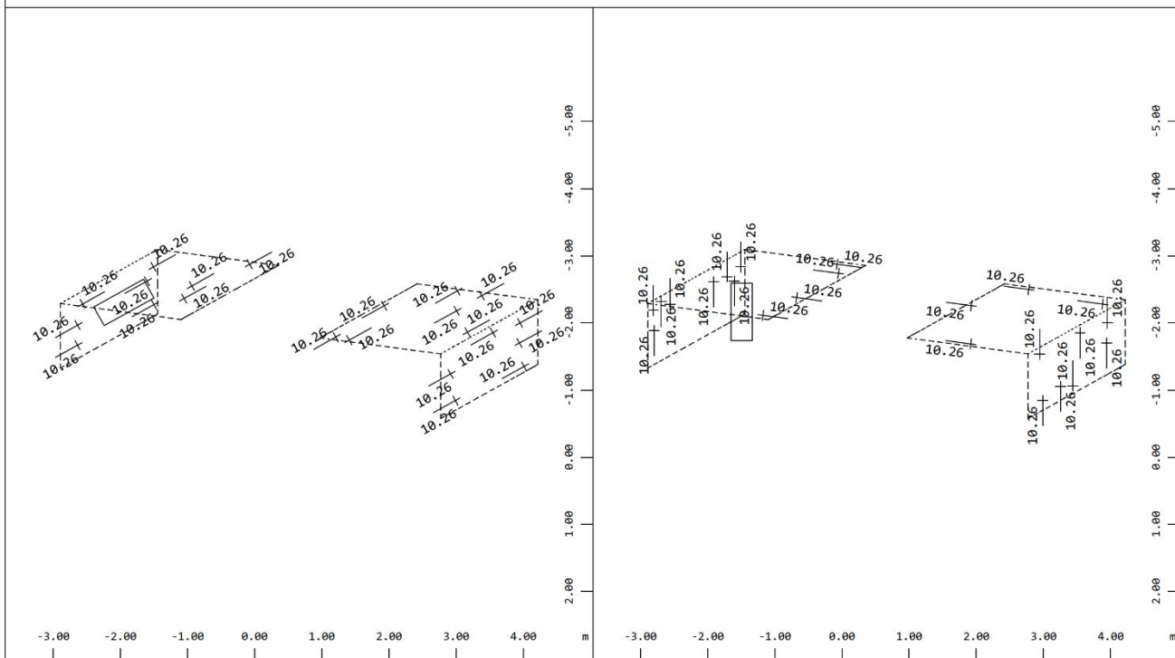
Sector of system Group 71 Quadrilateral Elements , upper Principal reinforcements (1st layer) in Node in cm 2 /m, Design Case 1 (Max=10.26)
