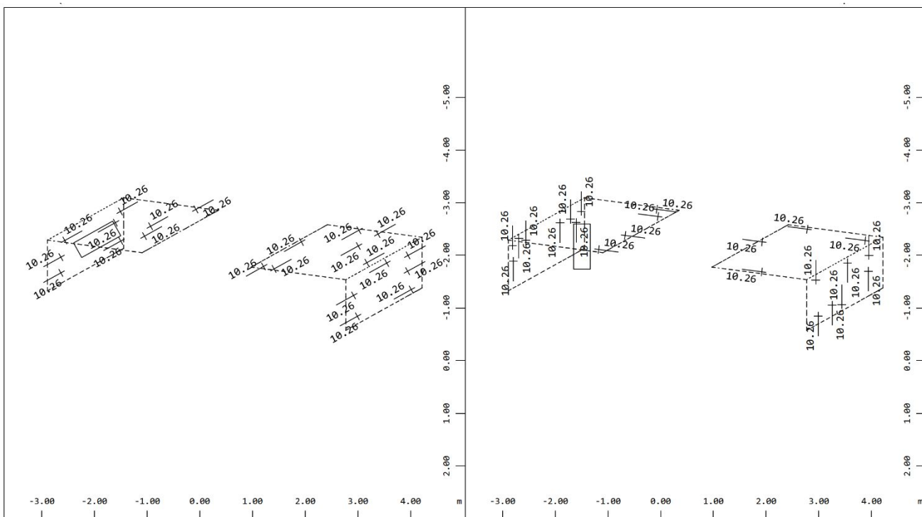
Sector of system Group 71 Quadrilateral Elements , lower Principal reinforcements (1st layer) in Node in cm 2 /m, Design Case 1 (Max=10.26)
